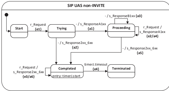
Fig. 4. Statecharts model of SIP UAS non-INVITE reusable test module
